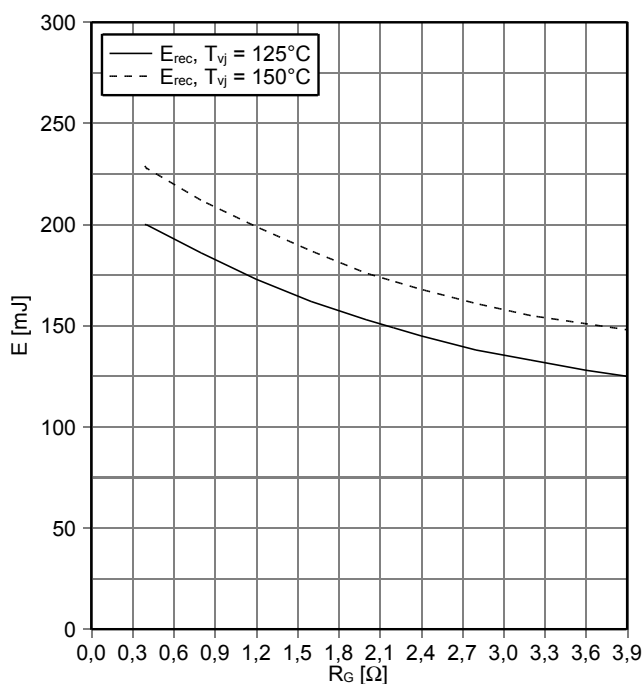
Schaltverluste Diode, Revers (typisch) switching losses Diode, Reverse (typical) E_{rec} = f(R_G) I_F = 800 A , V_{CE} = 900 V
