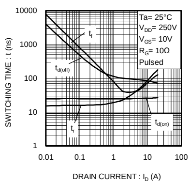
Fig.14 Switching Characteristics
