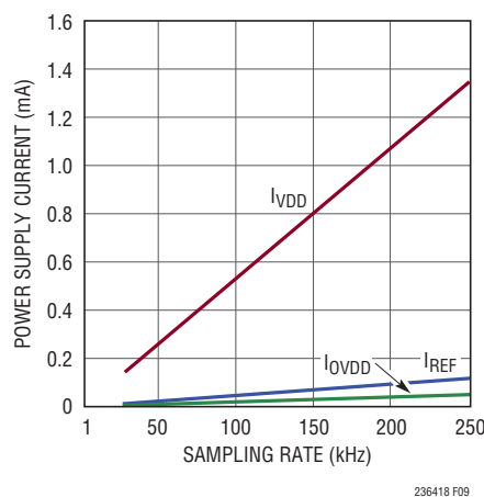
Figure 9. Power Supply Current of the LTC2364-18 Versus Sampling Rate
