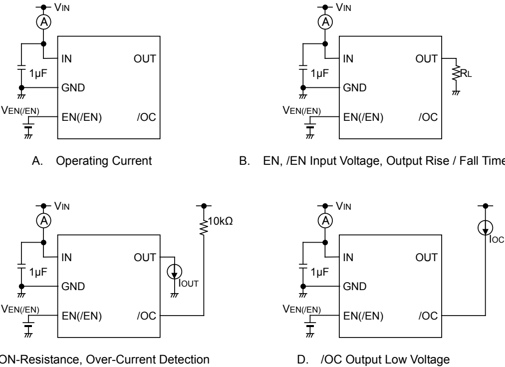
Figure 1. Measurement Circuit
