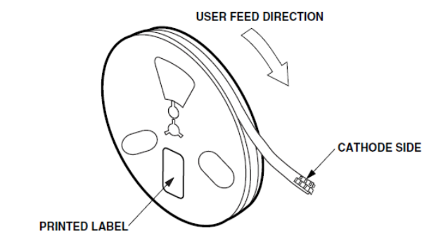
Figure 12: Reel Orientation
