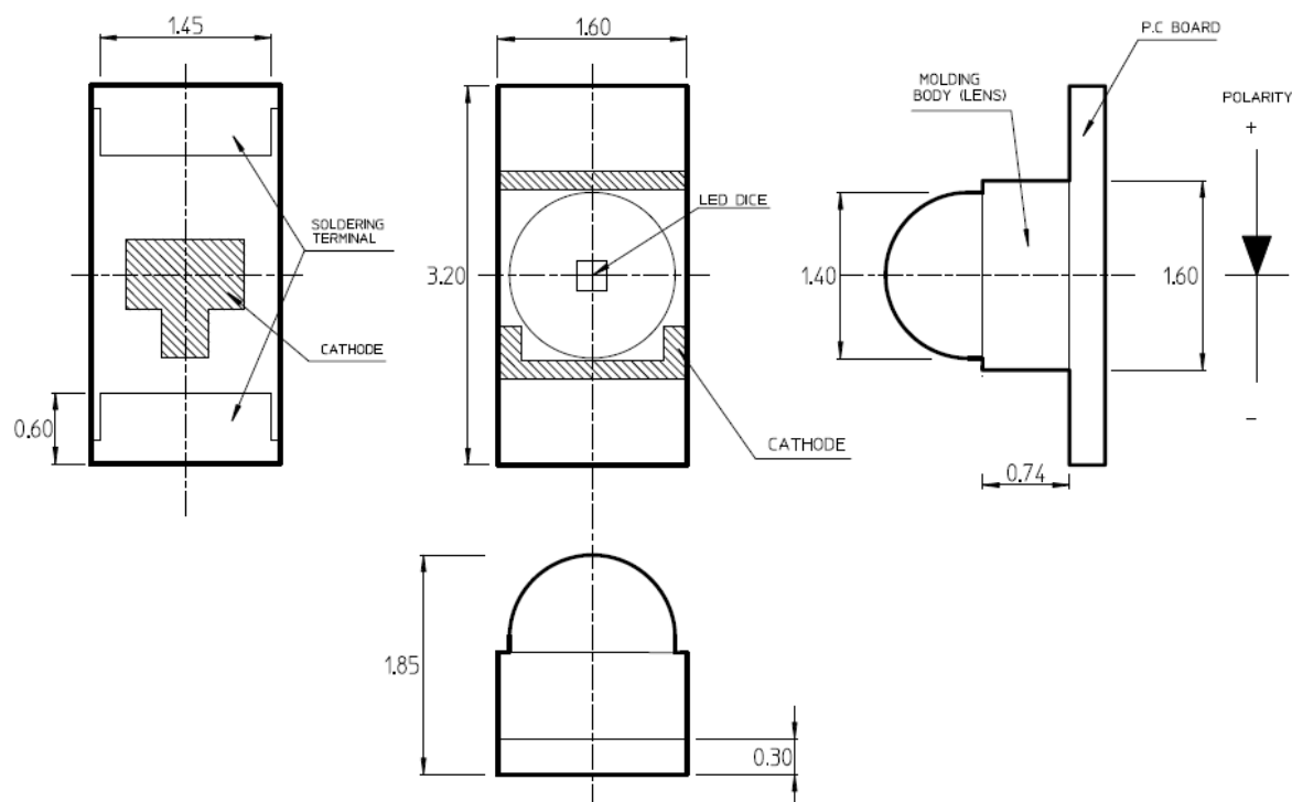
Figure 1: Package Dimensions
