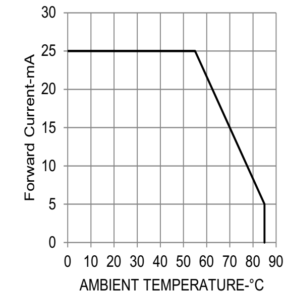
Figure 10: Derating Curve
