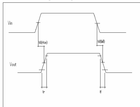
Timing diagram
