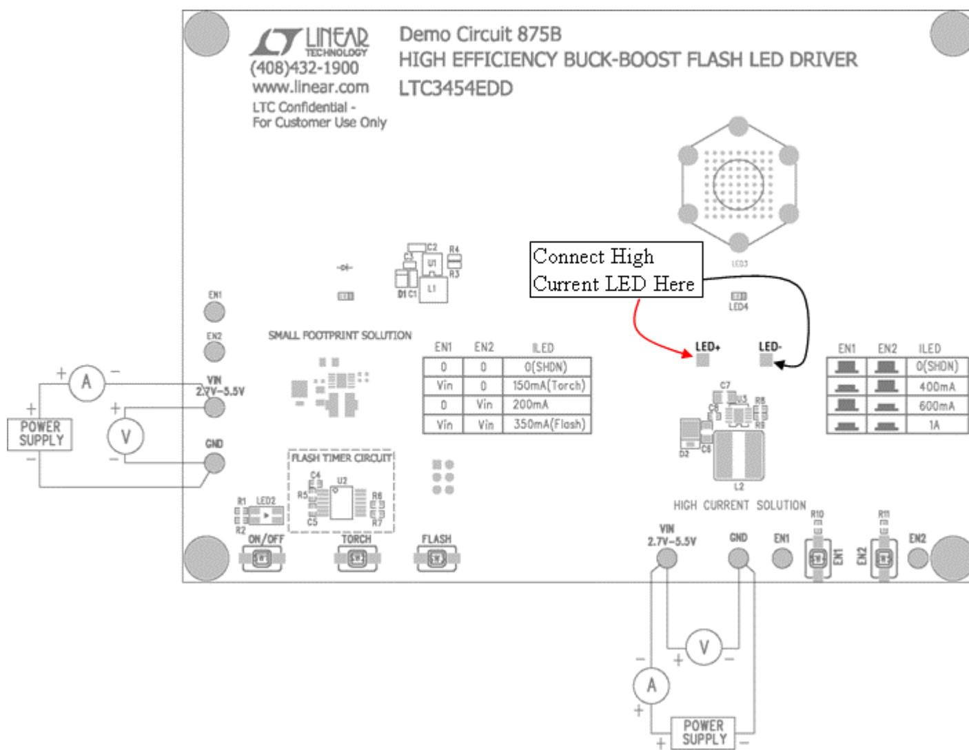
Figure 1. Proper Measurement Equipment Set
