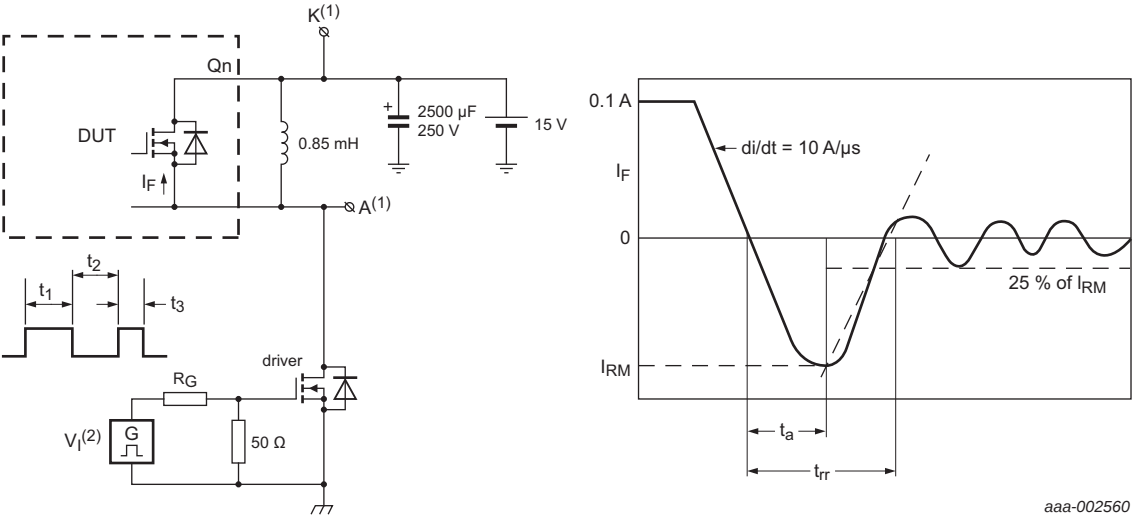
(1) The open-drain Qn terminal under test is connected to testpoint K. All other terminals are connected together and connected to testpoint A. (2) The V_I amplitude and R_G are adjusted for di/dt = 10 \text{ A}/\mu\text{s} . A V_I double-pulse train is used to set I_F = 0.1 \text{ A} , where t_1 = 10 \mu\text{s} , t_2 = 7 \mu\text{s} and t_3 = 3 \mu\text{s} .
