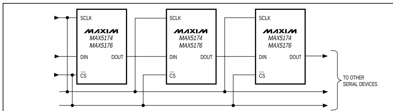
Figure 9. Daisy-Chaining MAX5174/MAX5175 Devices
