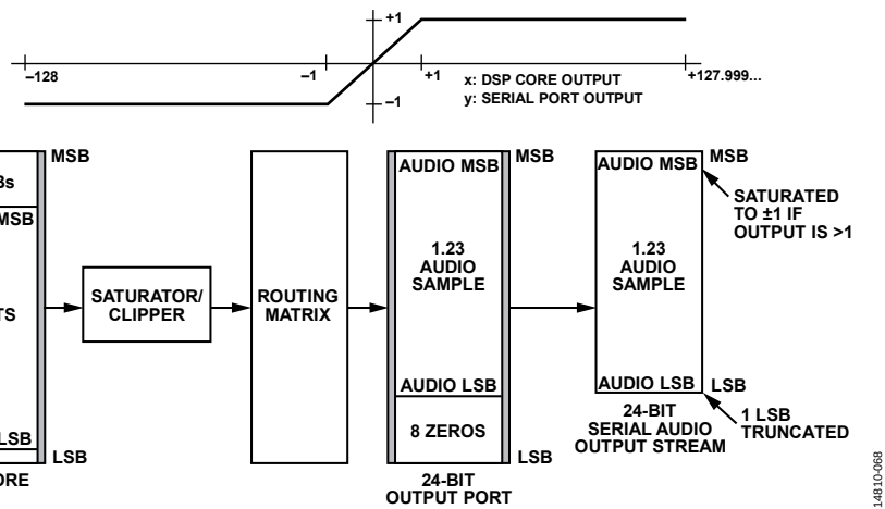
Figure 70. 24-Bit Serial Output Example
