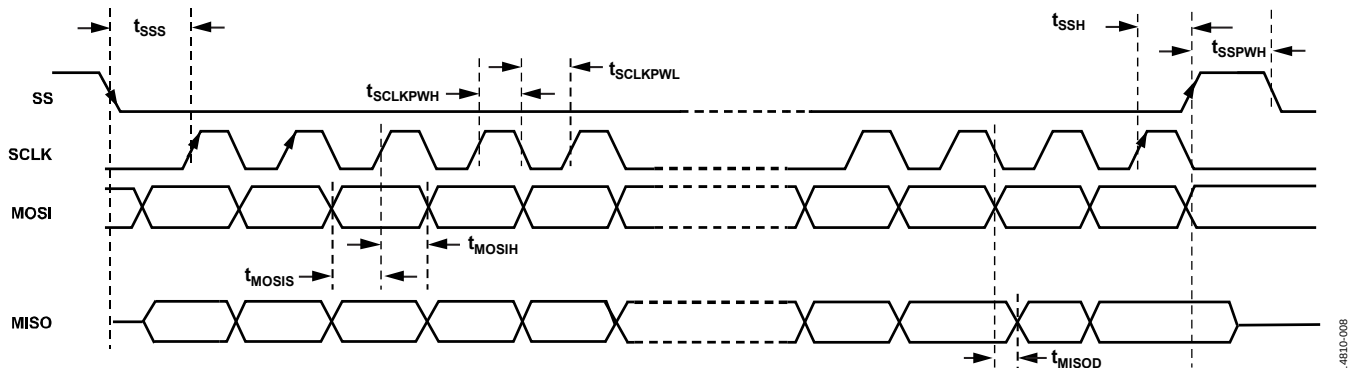
Figure 8. SPI Slave Port Timing Specifications
