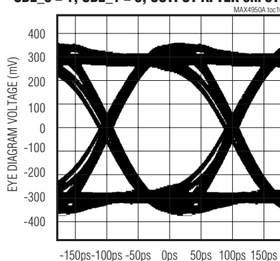
INEQ_0 = INEQ_1 = 0, O_AMP_ = 1, V_{IN} = 200mV_{p-p} , ODE_0 = 1, ODE_1 = 0, OUTPUT AFTER 6in STRIPLINE
