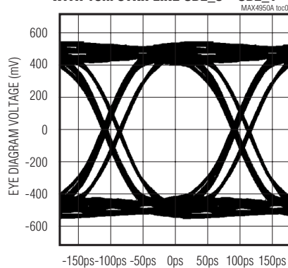
INEQ_0 = 0, INEQ_1 = 1, O_AMP_ = 0, V_{IN} = 500mV_{p-p} , WITH 19in STRIPLINE ODE_0 = ODE_1 = 0
