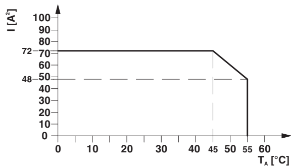
Figure 2 Derating curve
