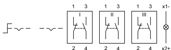
35 Selector switch 2 positions page 11 | Selector switch actuator 2 positions, flush mounting page 19
