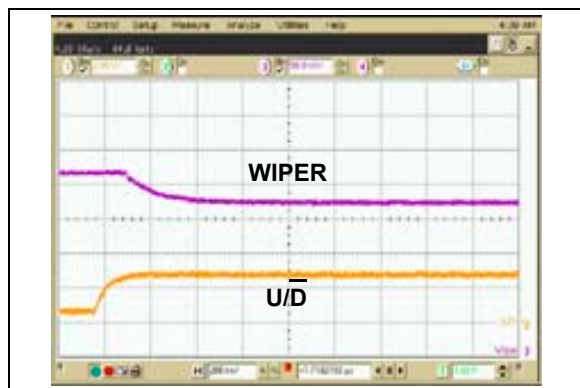
FIGURE 2-13: 2.1\text{ k}\Omega – Low-Voltage Decrement Wiper Settling Time ( V_{DD} = 2.7\text{V} ).
