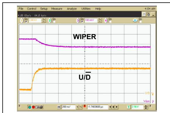
FIGURE 2-14: 2.1\text{ k}\Omega – Low-Voltage Decrement Wiper Settling Time ( V_{DD} = 5.5\text{V} ).
