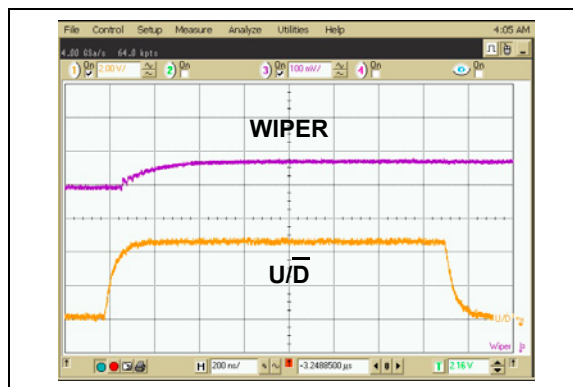
FIGURE 2-17: 2.1\text{ k}\Omega – Low-Voltage Increment Wiper Settling Time ( V_{DD} = 5.5\text{V} ).
