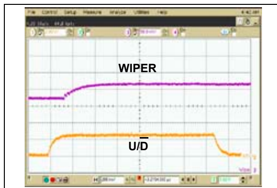
FIGURE 2-16: 2.1\text{ k}\Omega – Low-Voltage Increment Wiper Settling Time ( V_{DD} = 2.7\text{V} ).
