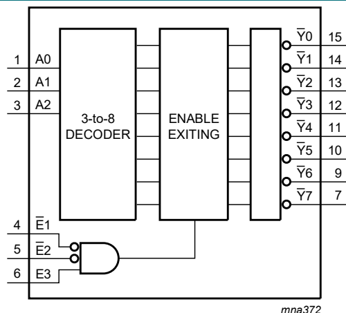
Fig. 2. Functional diagram
