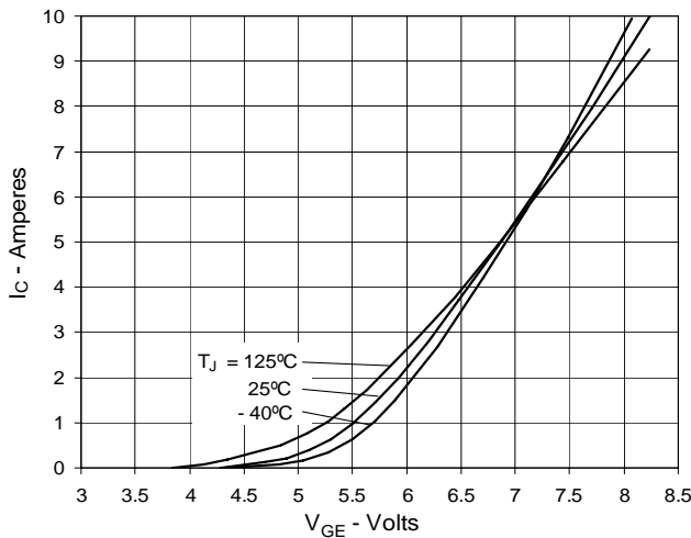
Fig. 5. Input Admittance
