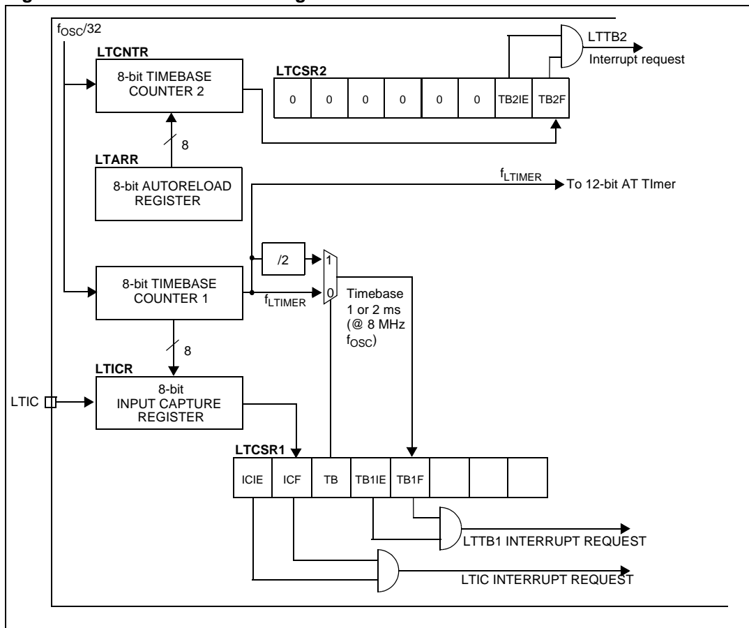
Figure 52. Lite timer 2 block diagram
