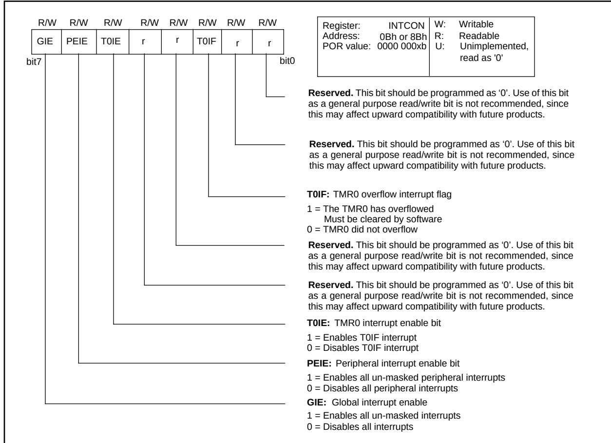
FIGURE 4-5: INTCON REGISTER
