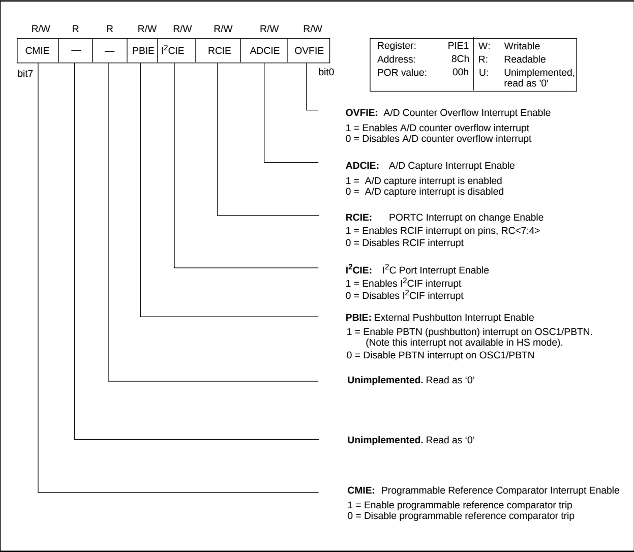
FIGURE 4-6: PIE1 REGISTER
