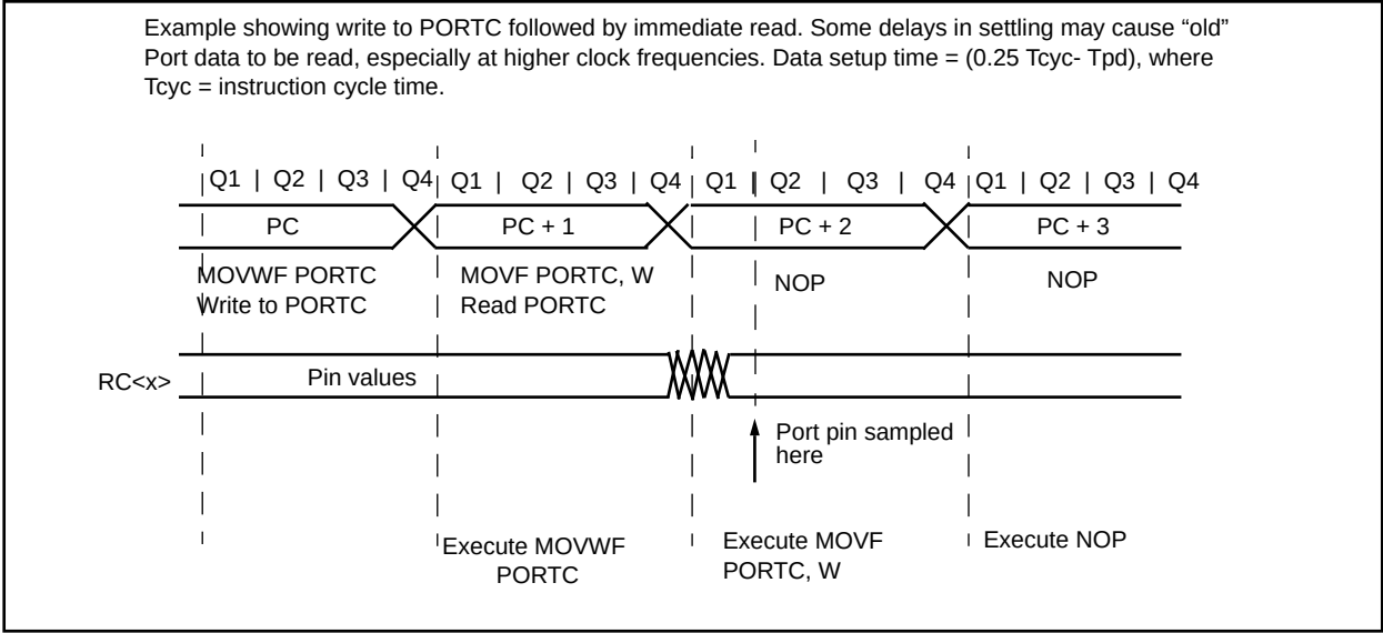
FIGURE 5-13: SUCCESSIVE I/O OPERATION
