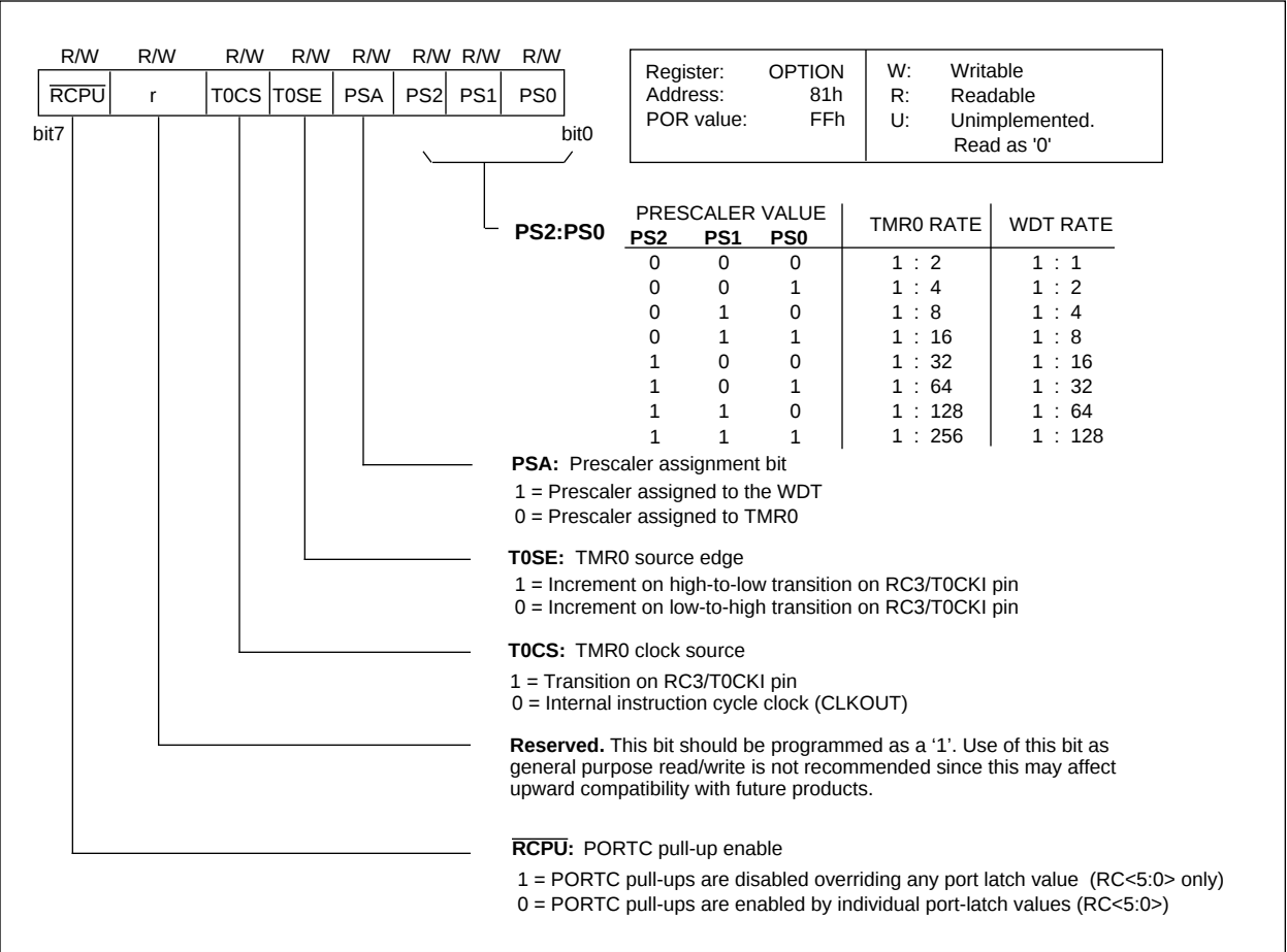
FIGURE 4-4: OPTION REGISTER
