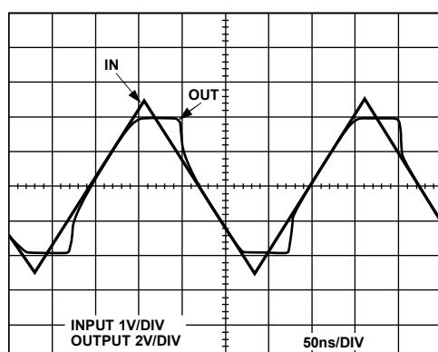
Figure 34. Output Overdrive Recovery, Gain = +2
