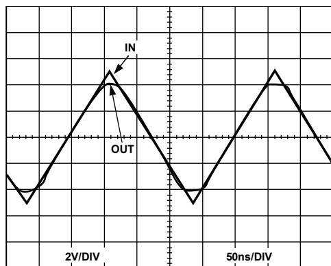
Figure 33. Input Overdrive Recovery, Gain = +1
