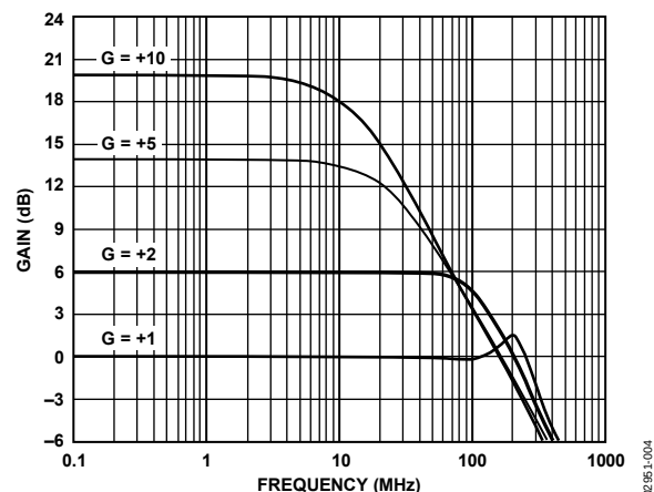
Figure 4. Small Signal Frequency Response for Various Gains, V_{OUT} = 500 \text{ mV p-p} , V_S = \pm 5 \text{ V}
