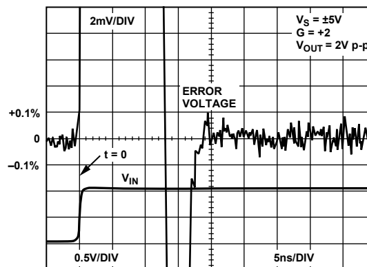
Figure 35. 0.1% Settling Time V_{OUT} = 2V p-p
