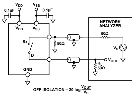
Figure 28. Off Isolation
