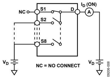
Figure 25. On Leakage
