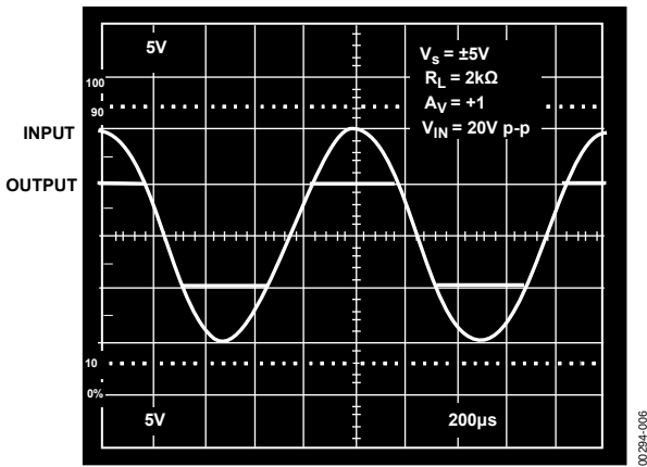
Figure 6. Input and Output with Inputs Overdriven by 5 V
