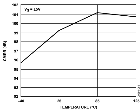
Figure 53. CMRR vs. Temperature, V_S = \pm 5 V
