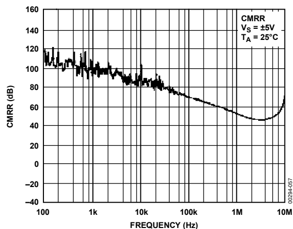
Figure 52. CMRR vs. Frequency, V_S = \pm 5 V
