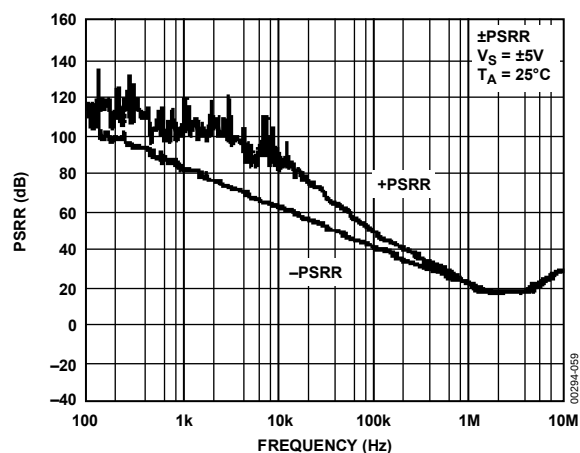
Figure 54. PSRR vs. Frequency, V_S = \pm 5 V
