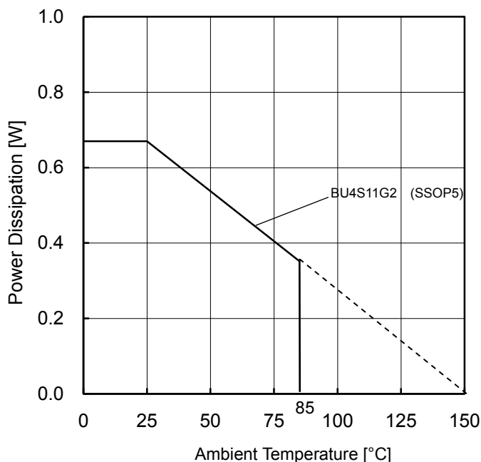
Figure 12. Derating Curve
