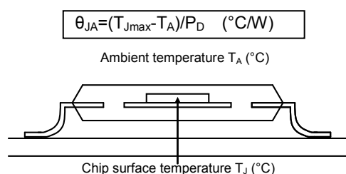
Figure 11. Thermal resistance
