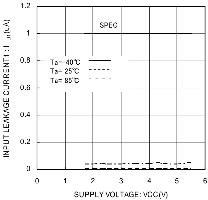
Figure 10. Input leakage current1 I_{IL1} (CS)
