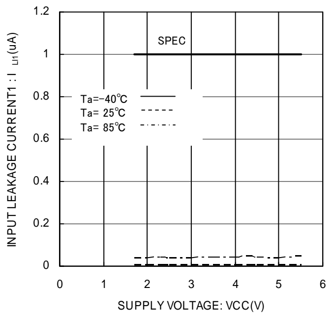
Figure 11. Input leakage current1 I_{IL1} (SK)
