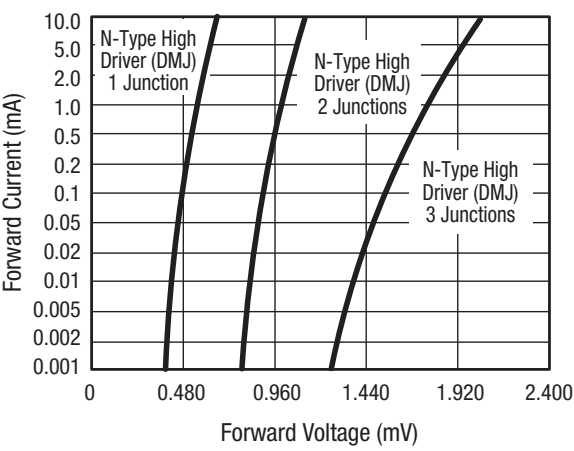
Figure 2. Typical Forward DC Characteristic Curves (Voltage vs current)
