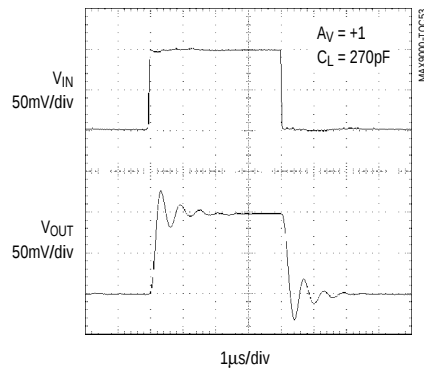
MAX9000/MAX9001/MAX9002 OP-AMP SMALL-SIGNAL TRANSIENT RESPONSE WITH C_{LOAD}
