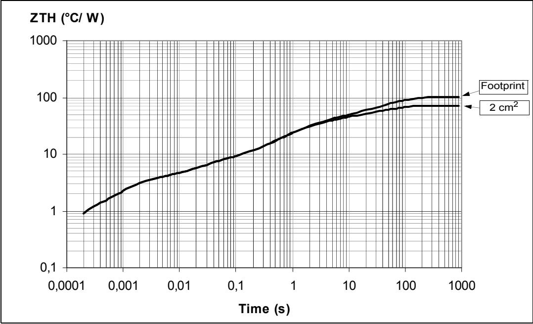
Figure 36. SO-8 thermal impedance junction ambient single pulse
