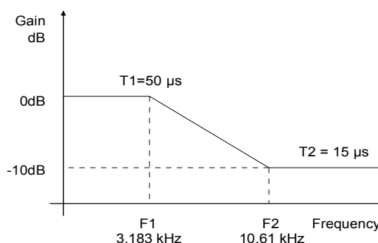
Figure 18. De-Emphasis Curve
