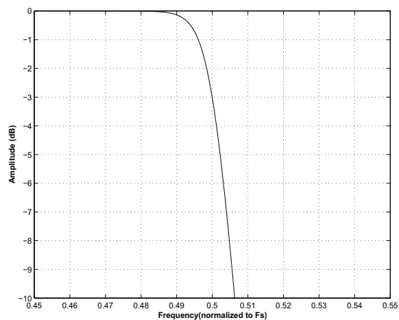
Figure 24. Single-Speed (fast) Transition Band (detail)
