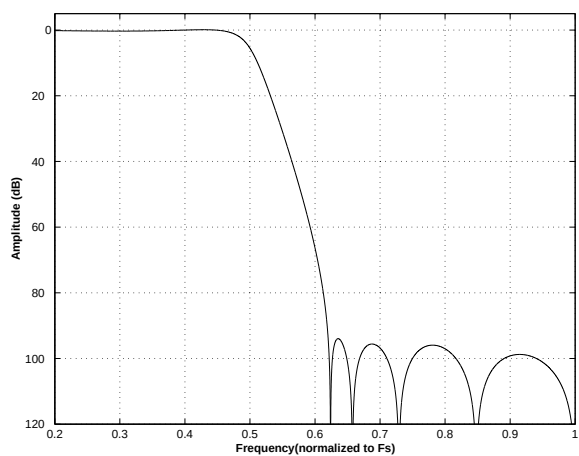
Figure 38. Quad-Speed (fast) Stopband Rejection
