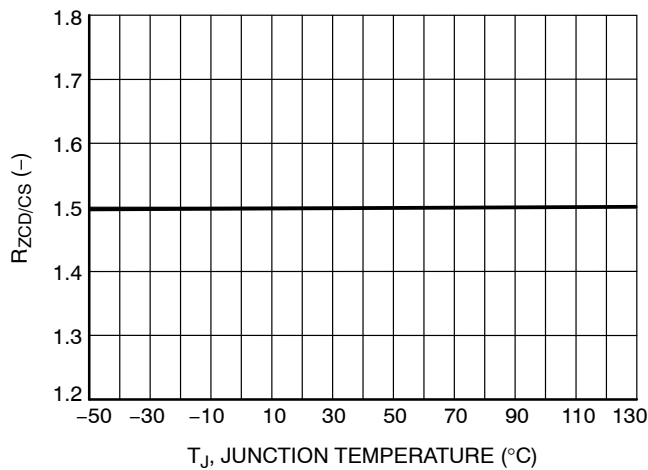
Figure 32. V ZCD(th) over V CS(th) Ratio vs. Temperature
