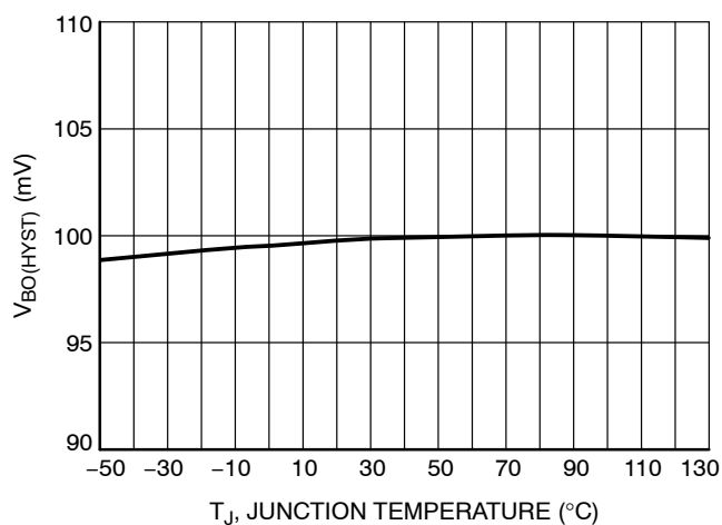
Figure 52. Brown-Out Comparator Hysteresis vs. Temperature
