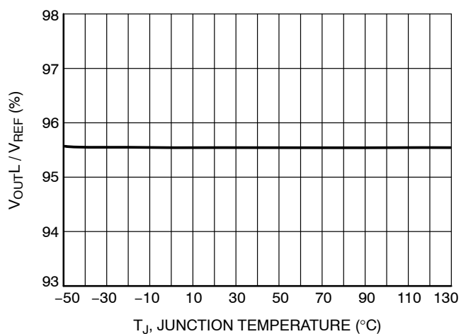
Figure 22. Ratio (V OUT Low Detect Threshold / V REF ) vs. Temperature
