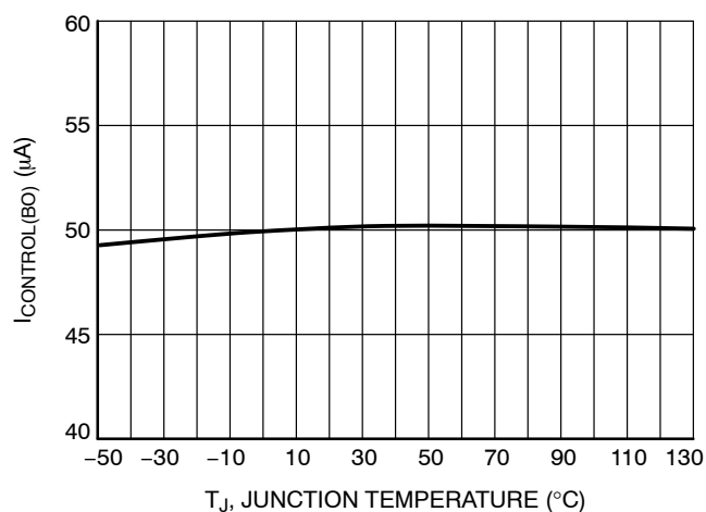
Figure 54. V_{CONTROL} Pin Sink Current when a Brown-Out Situation is Detected vs. Temperature
