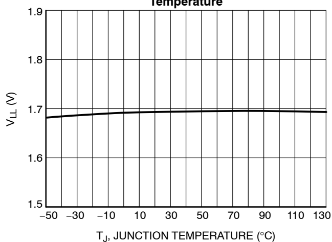
Figure 56. Comparator Threshold for Line Range Detection, V_{SENSE} Falling vs. Temperature
