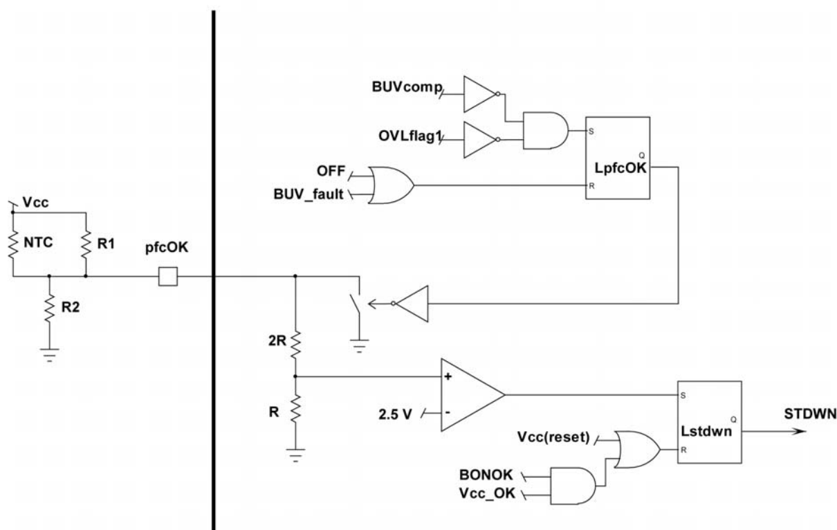
Figure 70. pfcOK Detection
