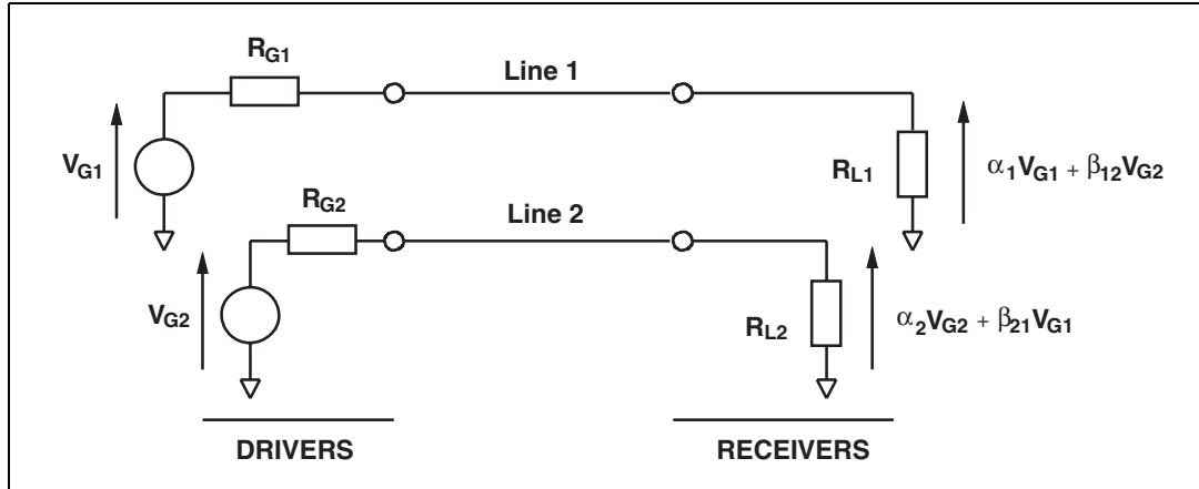
Figure 13. Crosstalk phenomena
