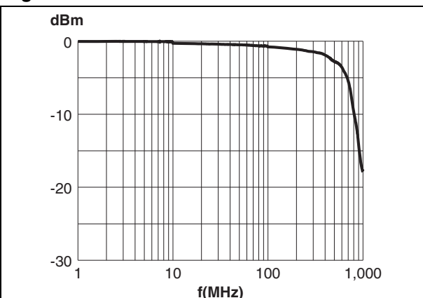
Figure 18. DALC208SC6 attenuation
