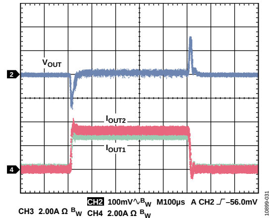
Figure 33. Load Transient, Channel 1/Channel 2 Parallel Output, 0 A to 6 A, V_{IN} = 12\text{ V} , V_{OUT} = 3.3\text{ V} , f_{SW} = 600\text{ kHz} , L = 4.7\text{ }\mu\text{H} , C_{OUT} = 47\text{ }\mu\text{F} \times 4
