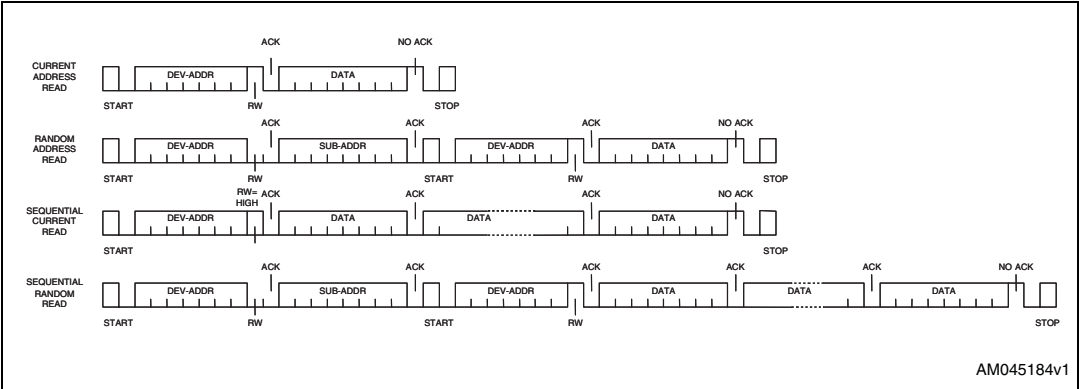
Figure 22. Read mode sequence
