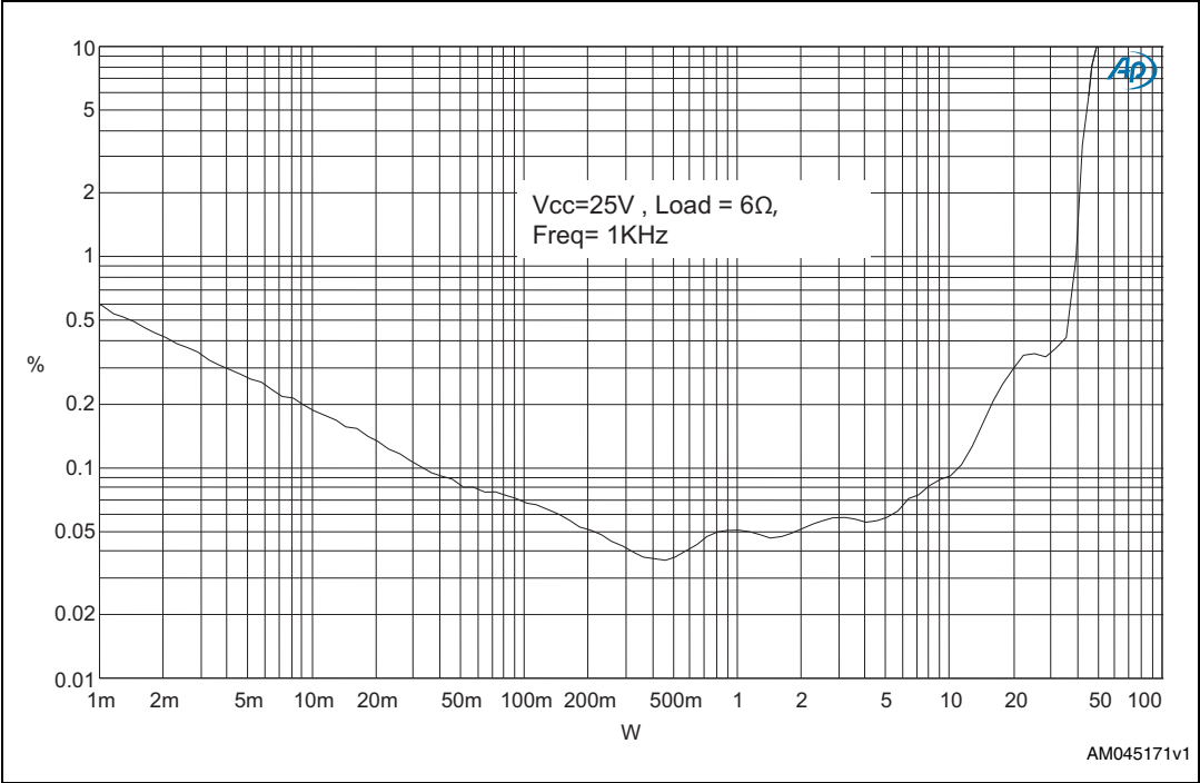
Figure 8. THD+N vs. output power ( V_{CC} = 25\text{ V} , load = 6\ \Omega )
