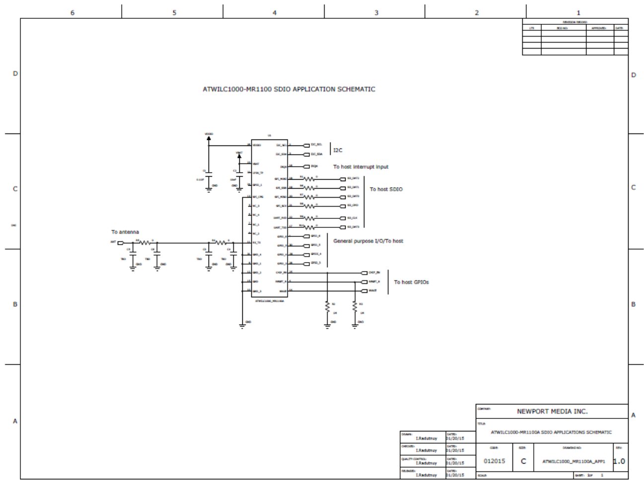
Figure 15-1. WILC1000-MR1100A SDIO
