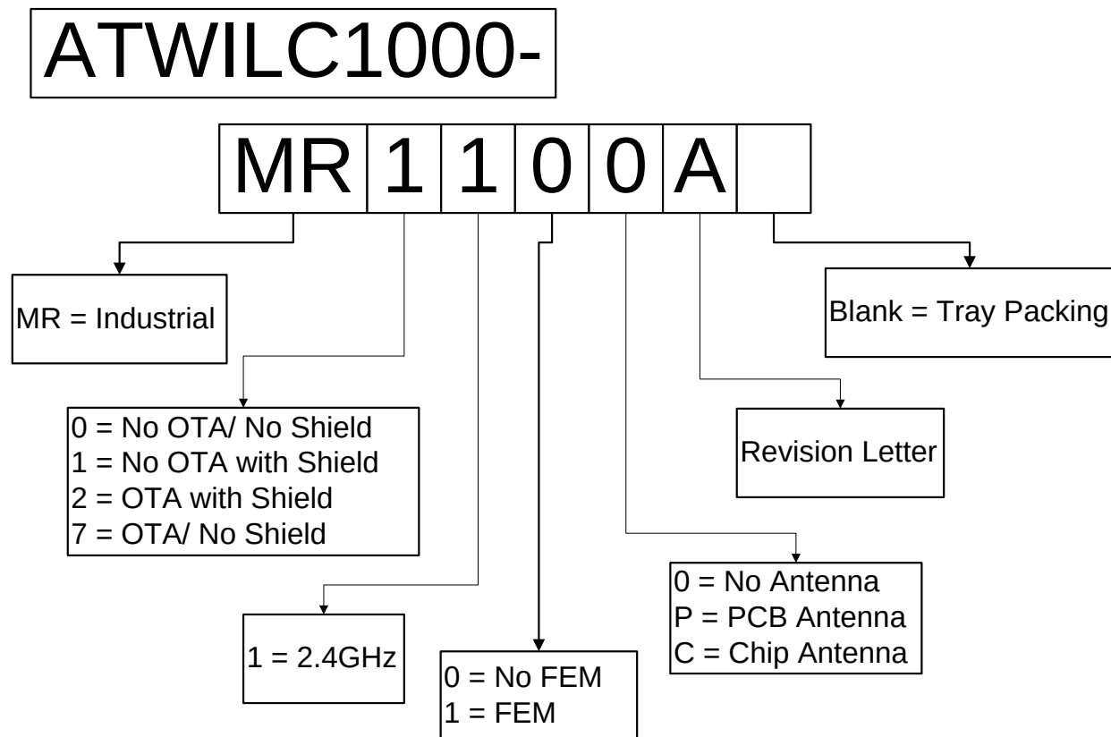
Figure 1-2. Marking Information
