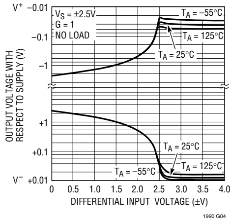
Output Voltage vs Input Voltage, G = 1
