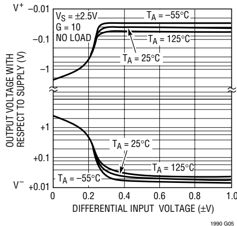
Output Voltage vs Input Voltage, G = 10
