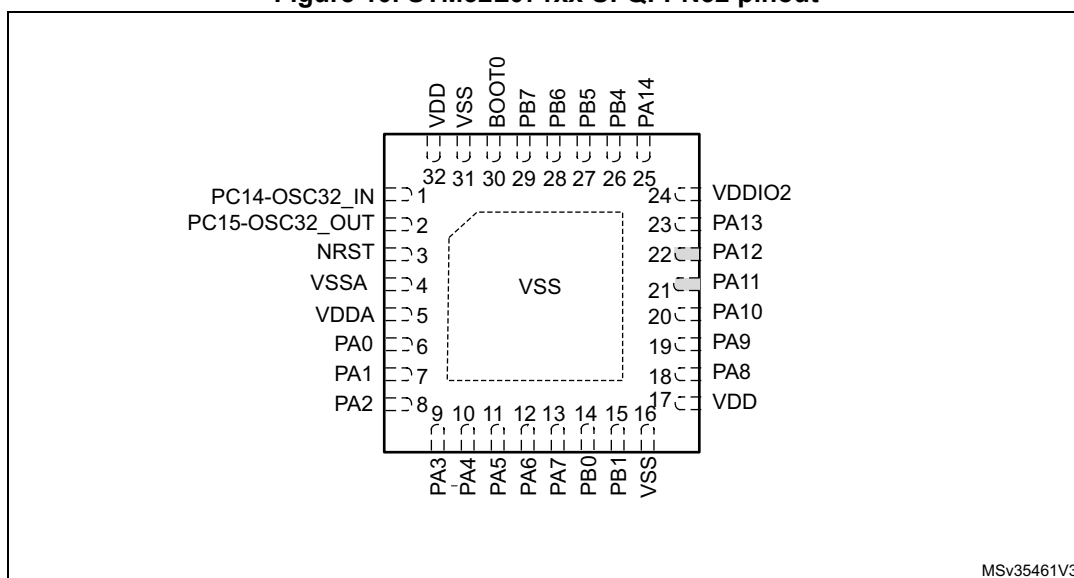
Figure 10. STM32L071xx UFQFPN32 pinout
