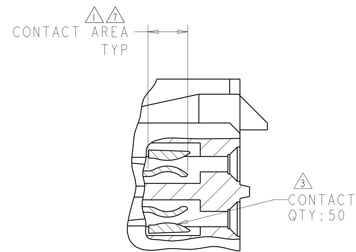
DETAIL M SCALE 12:1
