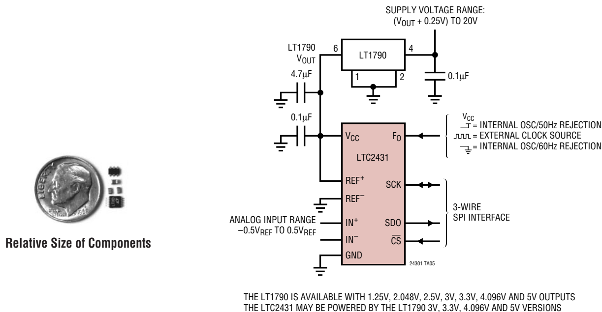
Figure 46. Complete 20-Bit Data Acquisition System in 0.1 inch 2
