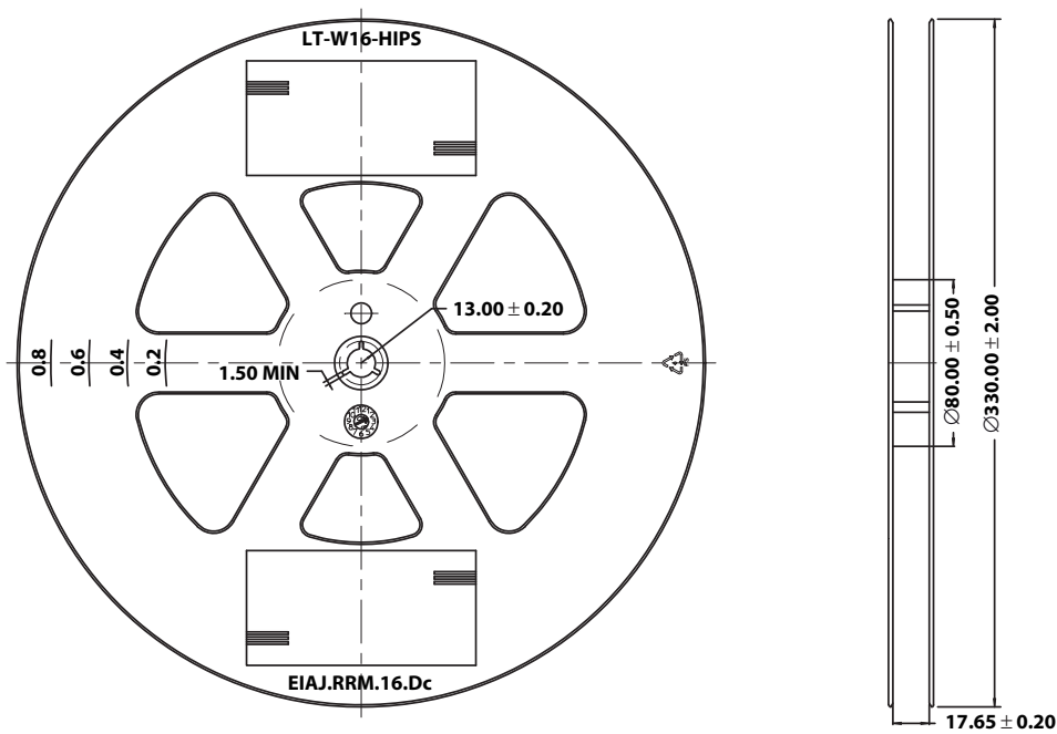
Figure 19. Reel Dimension
