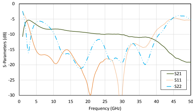
S-Parameters V_{C1} = -0.4\text{ V} , V_{C2} = -2.0\text{ V}
