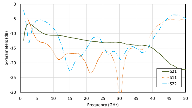
S-Parameters V_{C1} = -0.1\text{ V} , V_{C2} = -2.0\text{ V}
