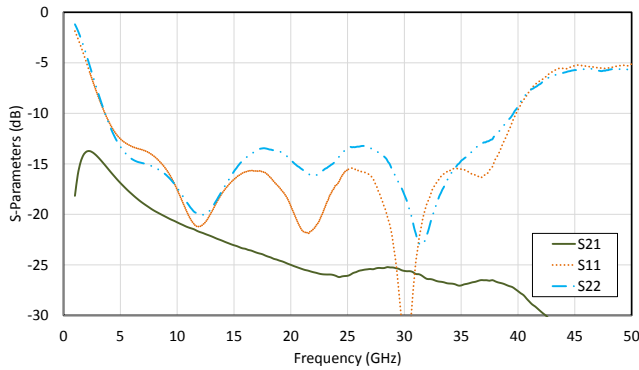
S-Parameters V_{C1} = 0\text{ V} , V_{C2} = -0.6\text{ V}
