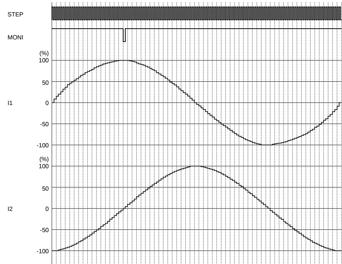
8W1-2 phase excitation (CW mode)
