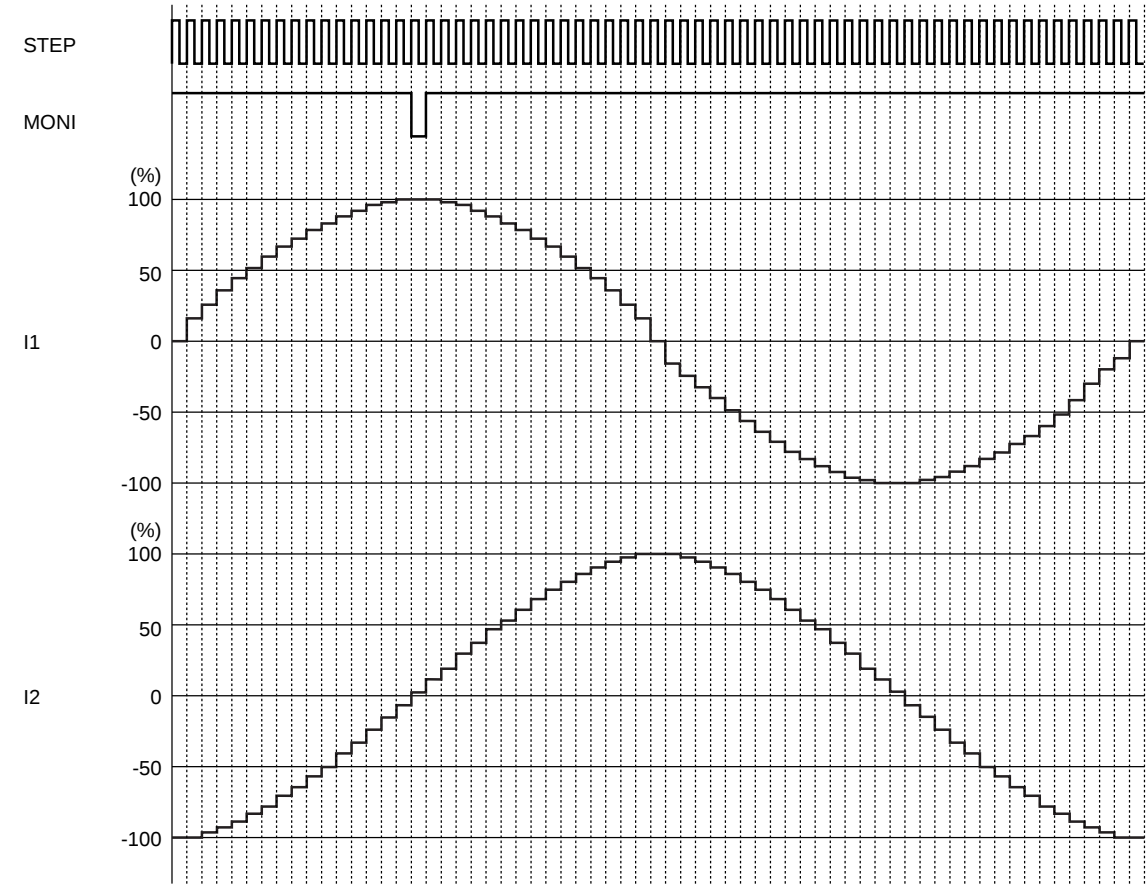
4W1-2 phase excitation (CW mode)
