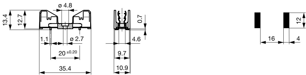
Solder pads
