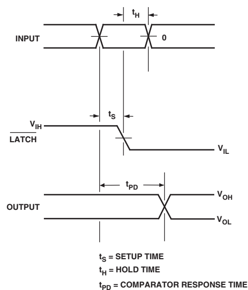
Figure 4. Latch Timing
