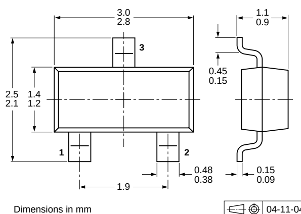
Fig 25. Package outline PDTD1xxxT series (SOT23/TO-236AB)
