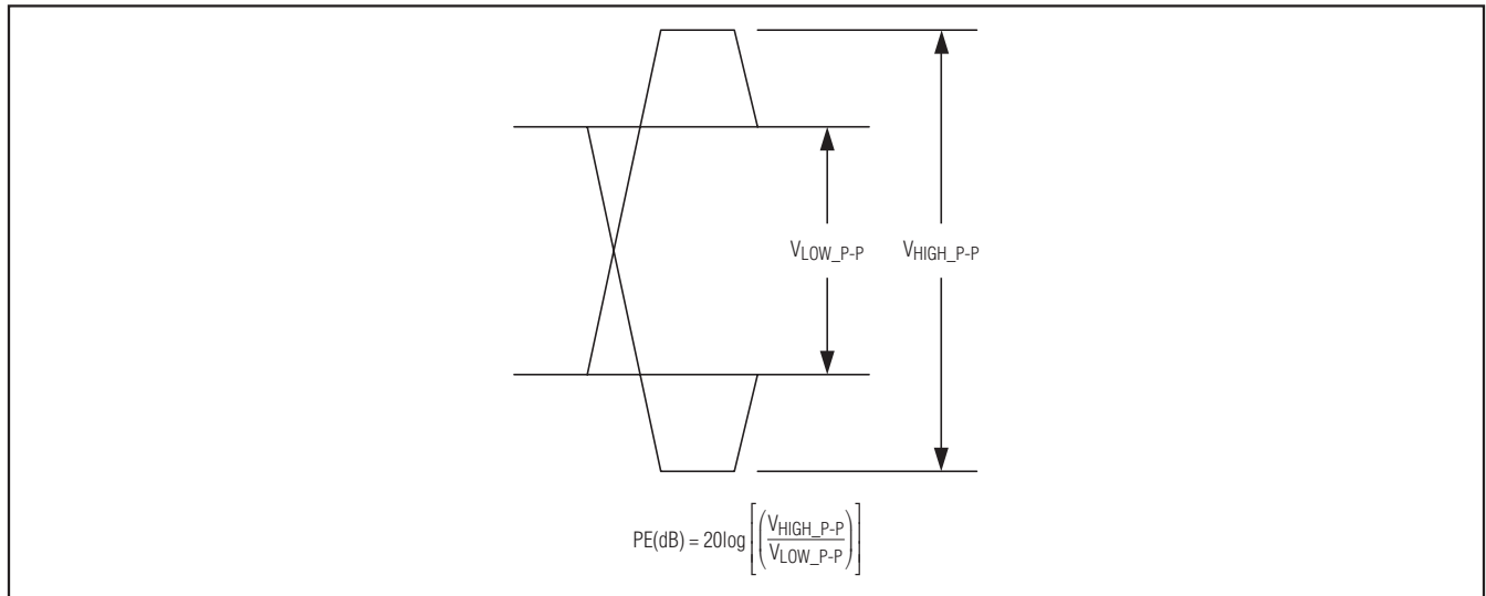
Figure 1. Output Preemphasis
