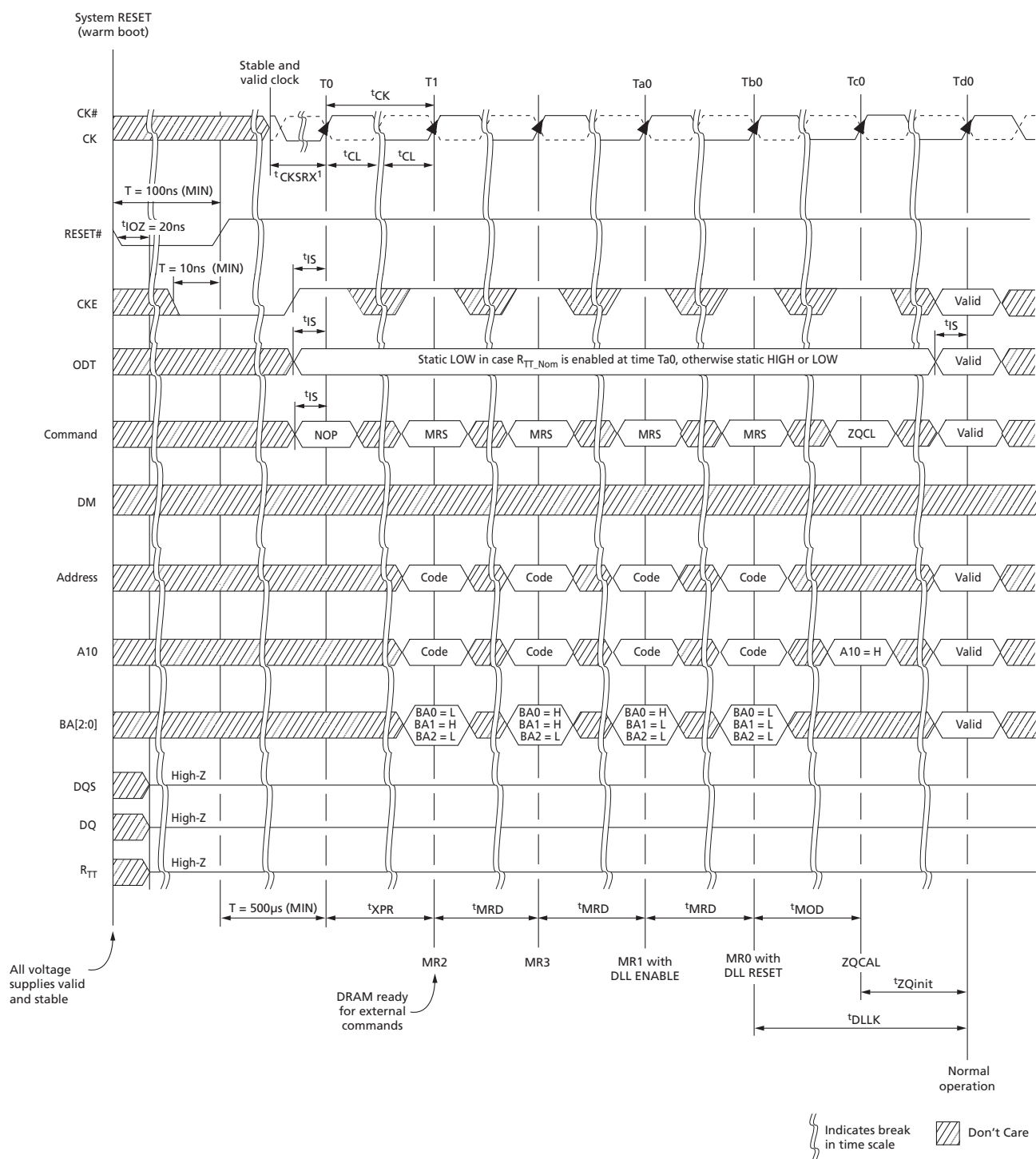
Figure 104: RESET Sequence
