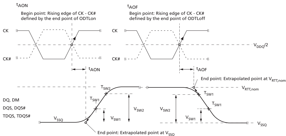
Figure 20: t_{AON} and t_{AOF} Definitions
