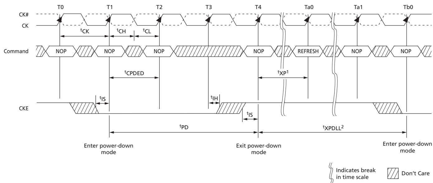
Figure 103: Power-Down Exit to Refresh to Power-Down Entry
